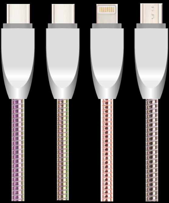
LM05-1019 USB AM- A:lightning 8P M B:Android Micro 5P M C:Type-C M Metal Shell +Metal spring
