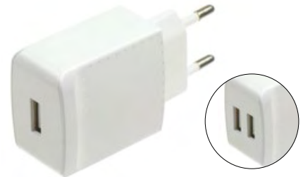
LM06-2020 QC3.0 Wall Charger Input: AC 110-240V Output: A: QC 3.0 18W B: 2*USB 2.0 5V 2.4A in Total
